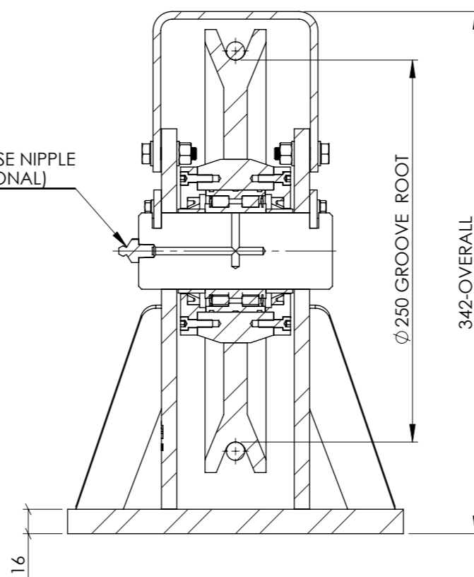
SECTION B-B
